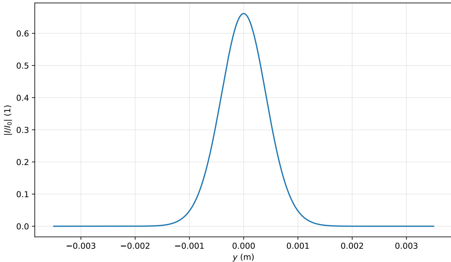
Intensity profile I(x=0, y, z=1.751)/I_0 , P_{in}=0.2P_{cr} , artificial time
